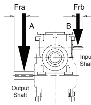
Double reduction (worm/worm)
